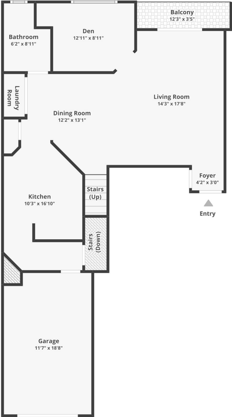
FLOOR 1
